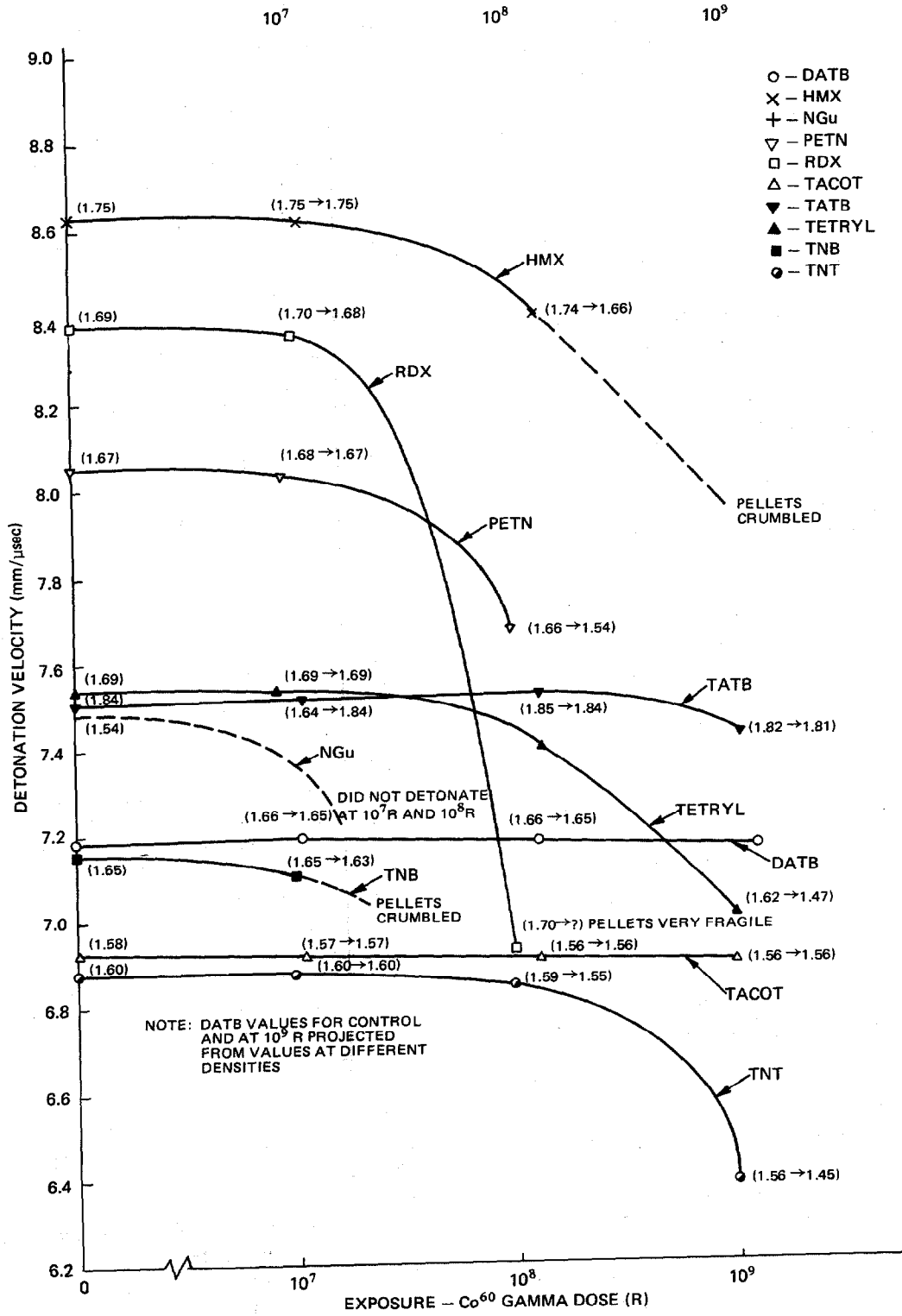
Fig 13 Effect of Gamma Radiation on the Detonation Velocity of Explosives (Ref 223)
